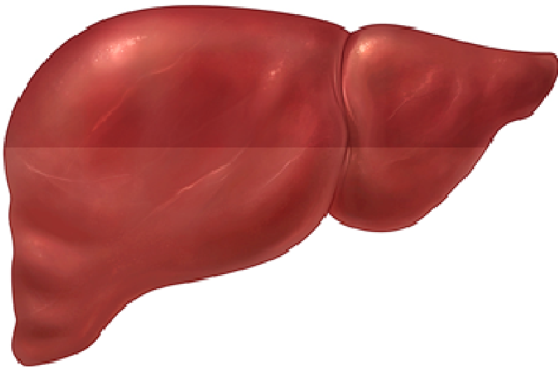
Normal Liver
